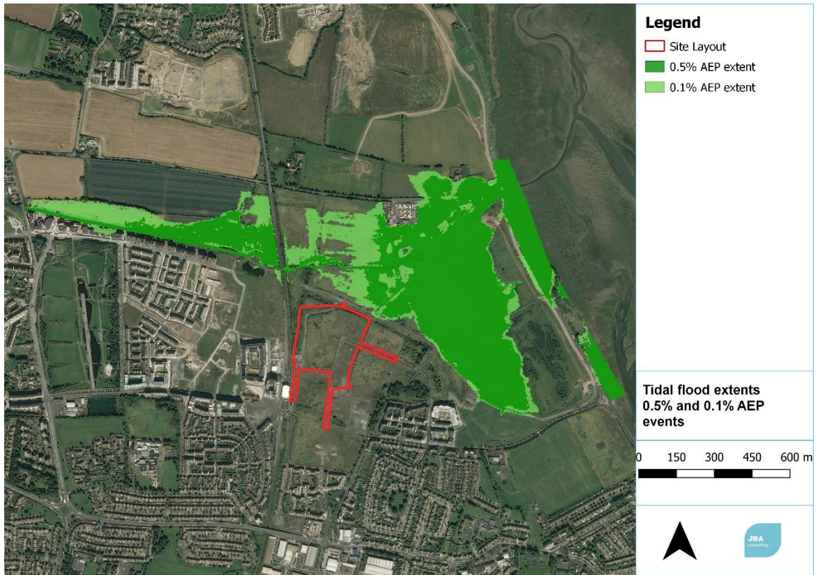
Figure 4-3: 0.5% and 0.1% AEP tidal flood extents - pre-development scenario
