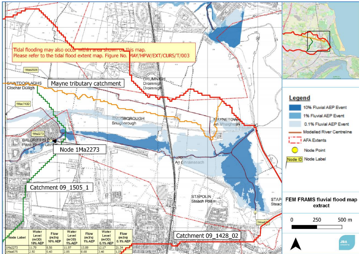
Figure 8-1: FEM FRAMS fluvial flood map extract
