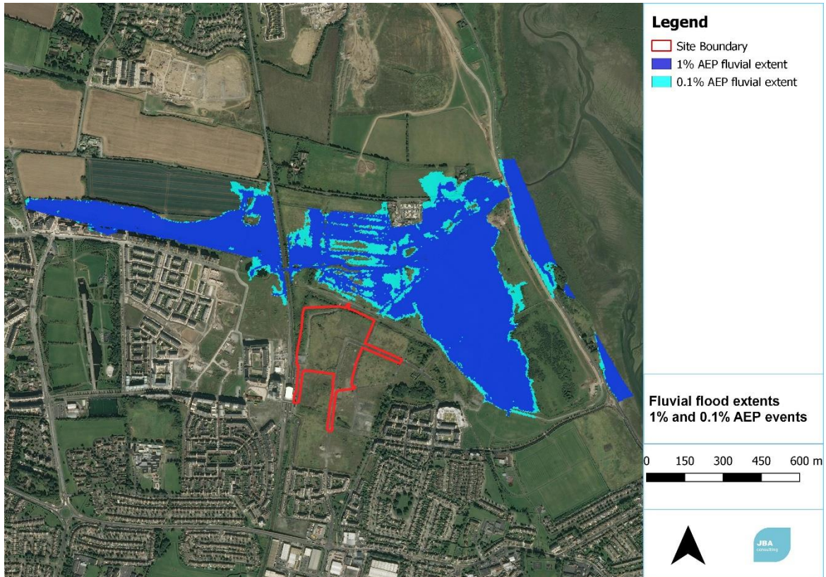
Figure 4-2: 1% and 0.1% AEP fluvial flood extents - pre-development scenario
